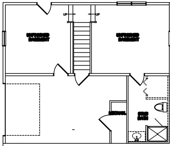
BASEMENT PLAN
